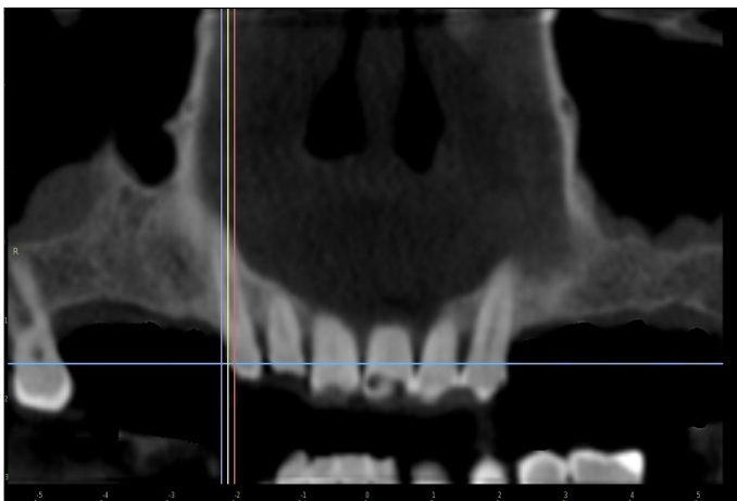
STANDARD CT SCAN
